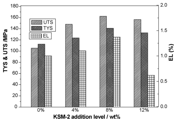
Fig. 12. Effect of KSM addition level on the tensile properties of GW103K alloy at room temperature.
