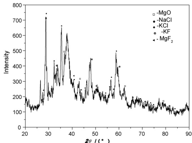
Fig. 15. XRD pattern of melting slag.
