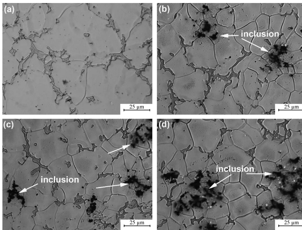
Fig. 8. Microstructure of GW103 alloy treated by KSM-3 with different addition level: (a) 0, (b) 4%, (c) 8% and (d) 12%.
